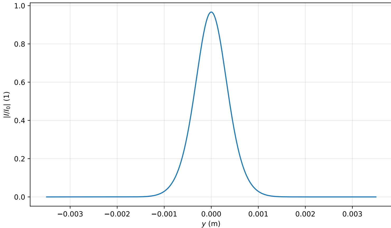
Intensity profile I(x=0, y, z=1.115)/I_0 , P_{in}=0.4P_{cr} , artificial time
